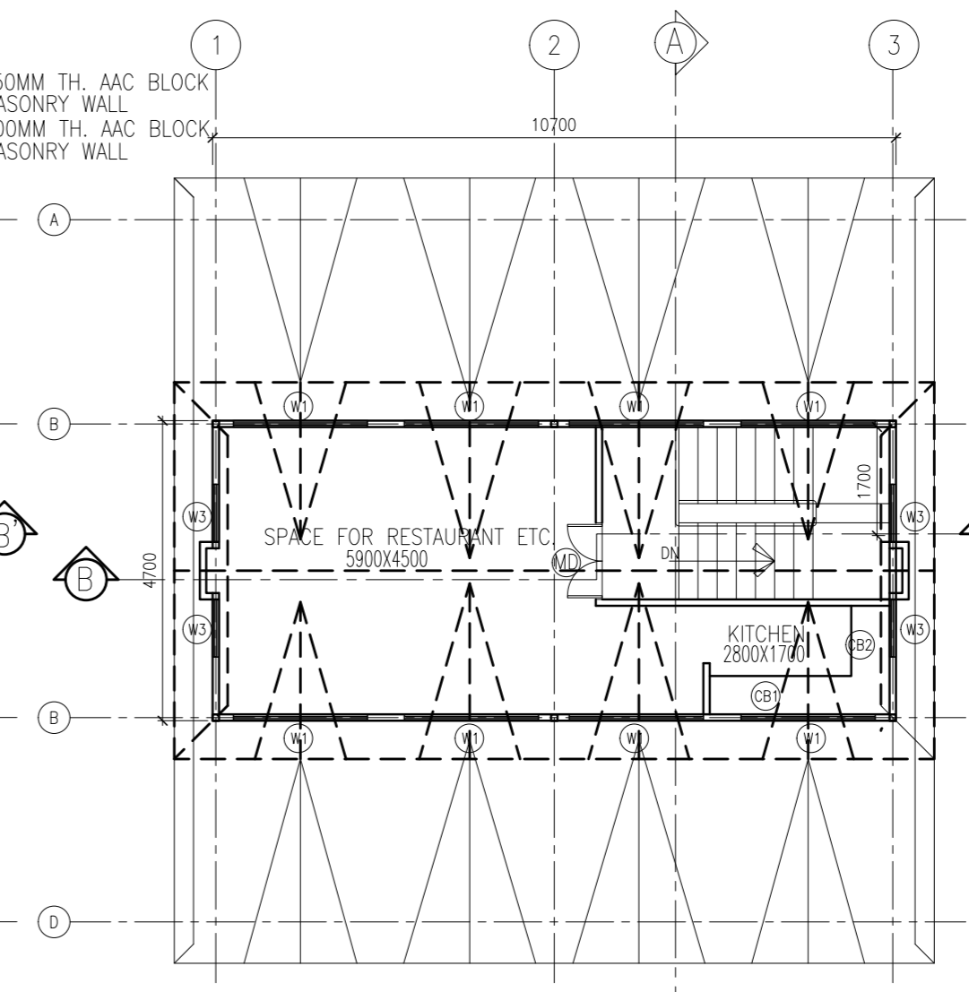
ATTIC/ ROOF PLAN SCALE 1:100
