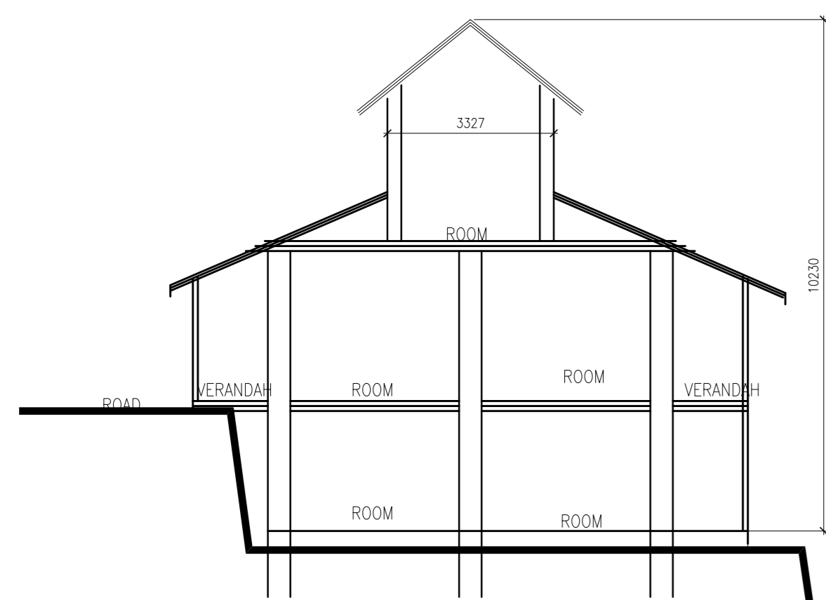
EXISTING BUILDING SECTION X-X SCALE 1:100
