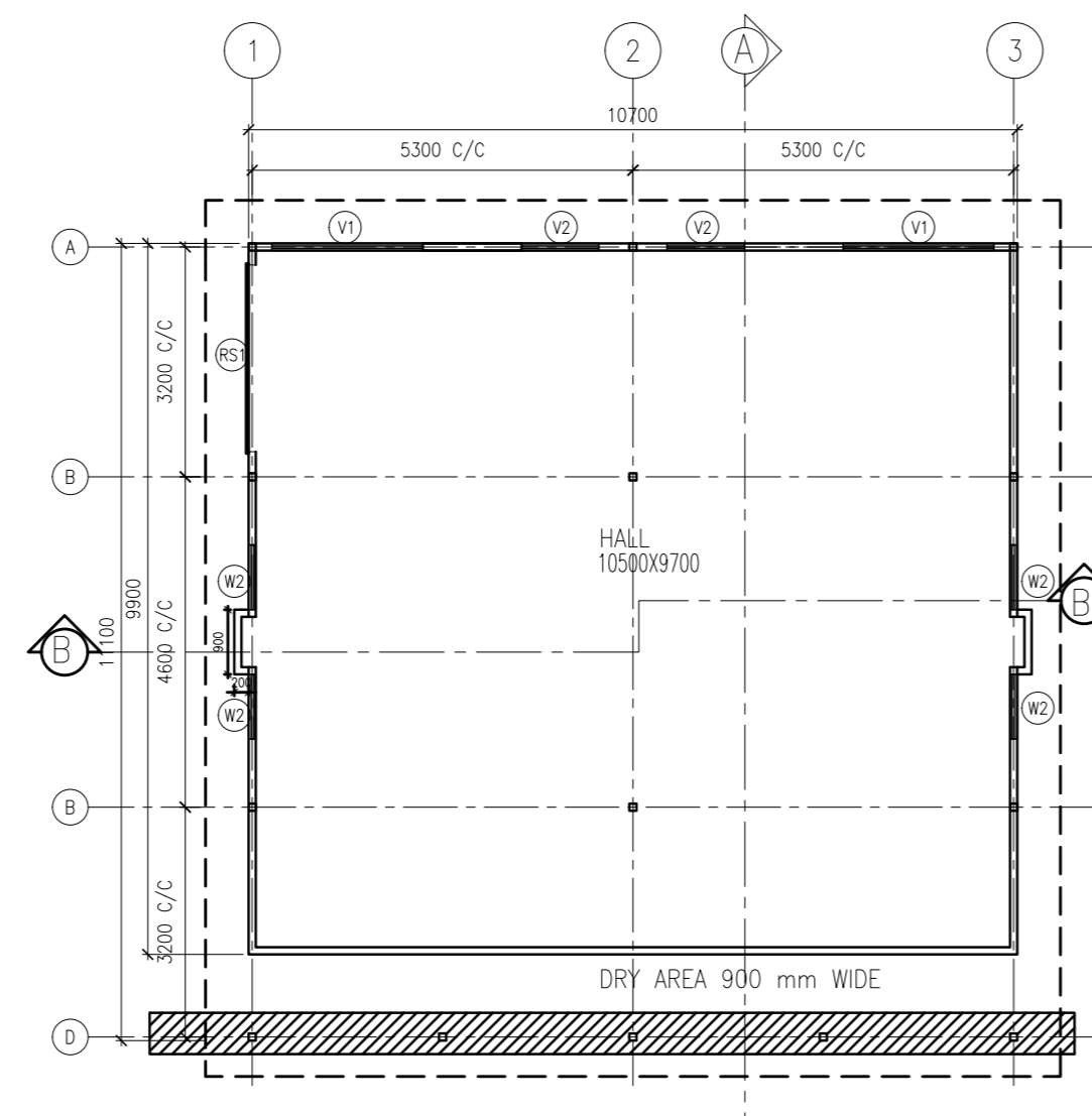
BASEMENT PLAN SCALE 1:100
