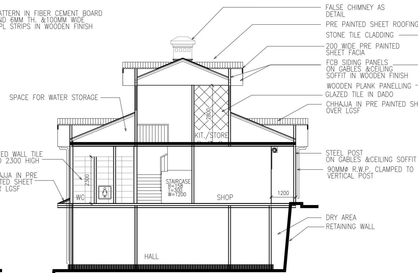
SECTION AT A-A' SCALE 1:100
