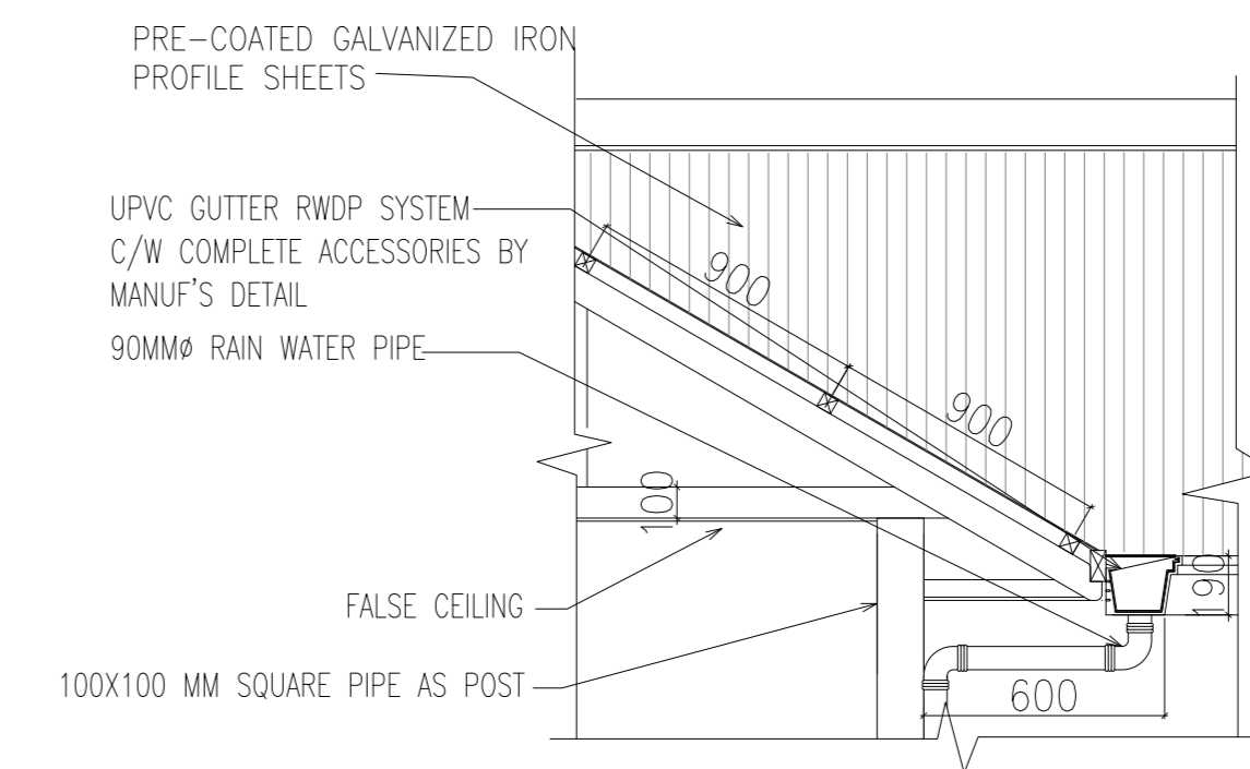
ROOF DETAIL SCALE 1:25
