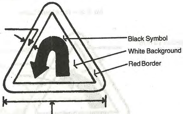
No. C 5 — Left Hair Pin Bend
