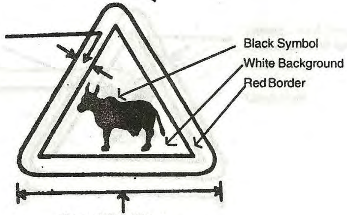
No. C 19 — Cattle
