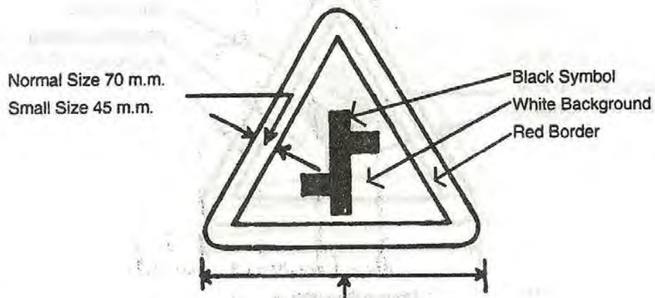
No. C 28A — Staggered Intersection
