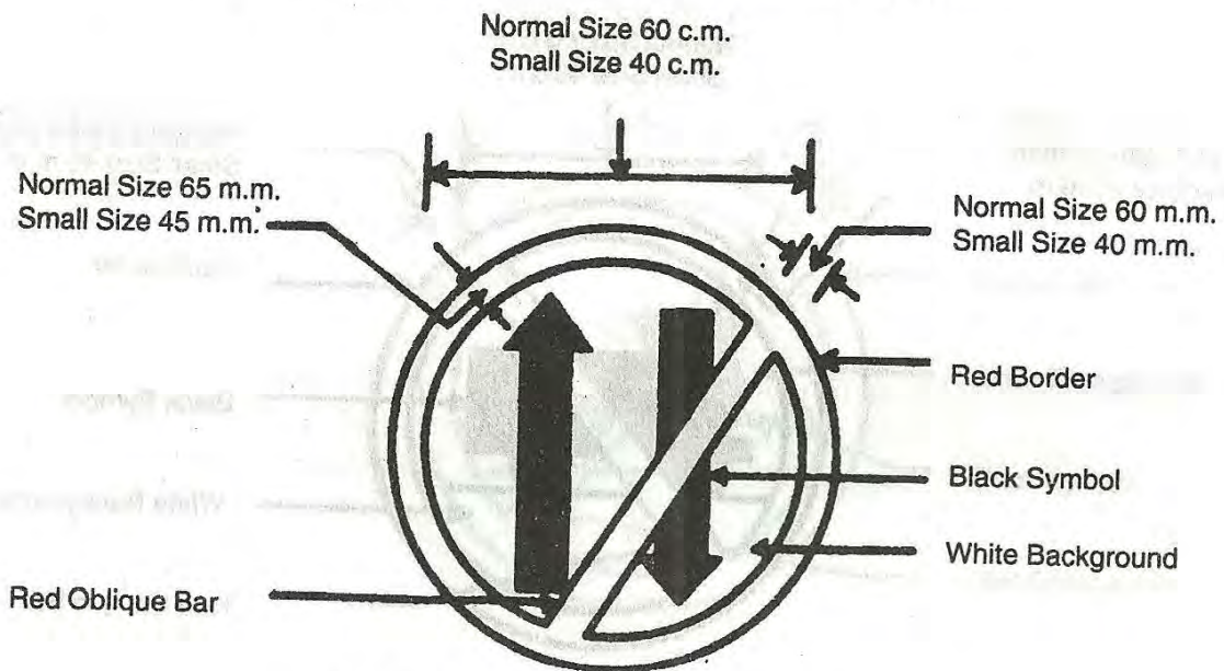
No. M 5 — Vehicles Prohibited in both Directions
