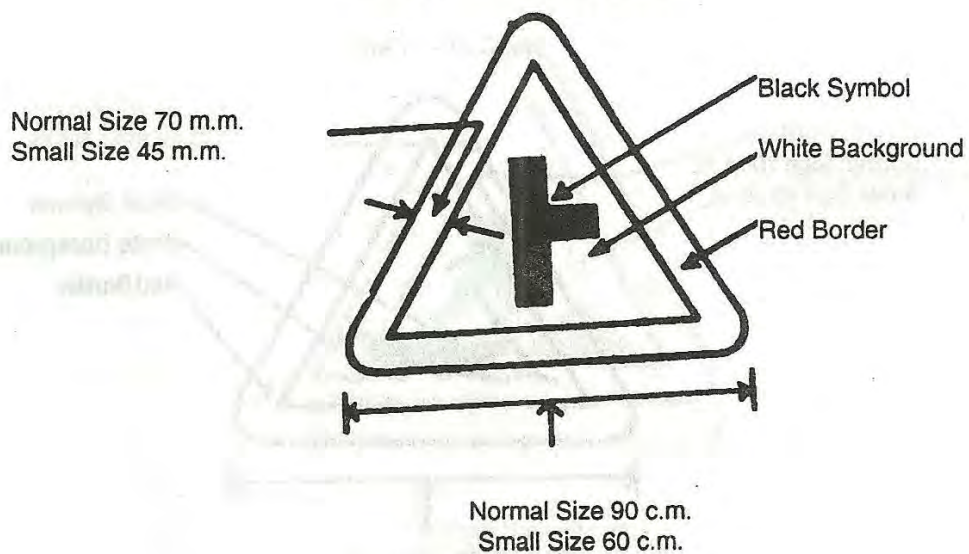
No. C 24 — Side Road Right
