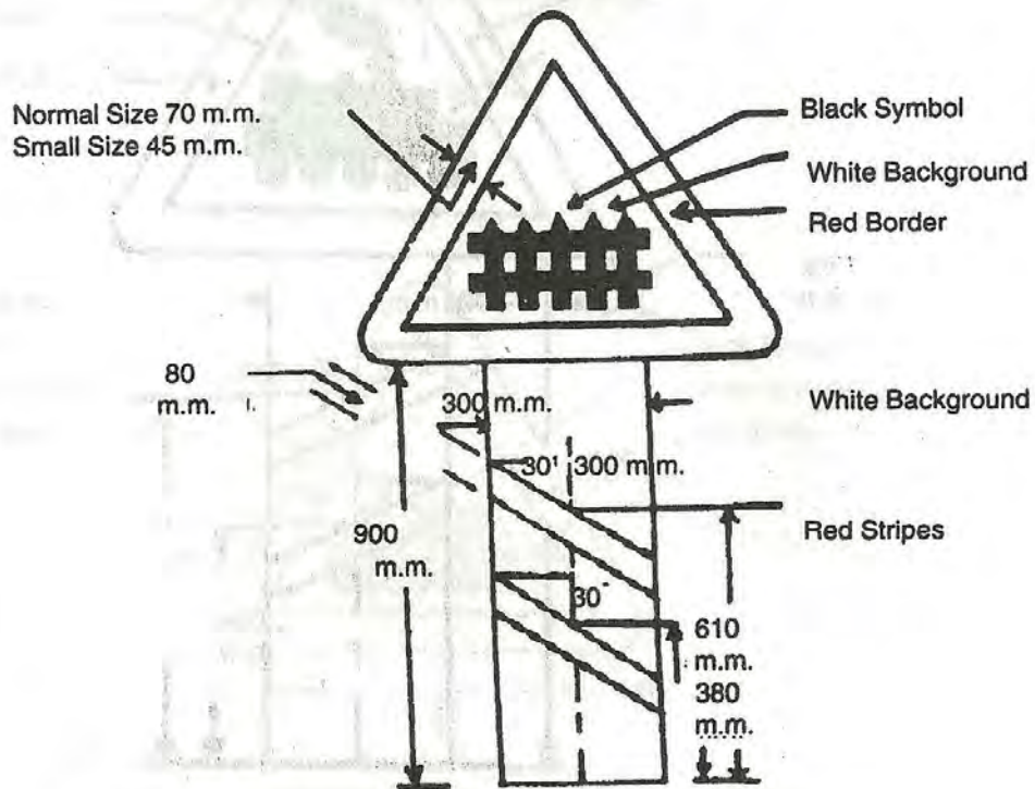
No. C 36 — Guarded Level Crossing (200 Metres)
